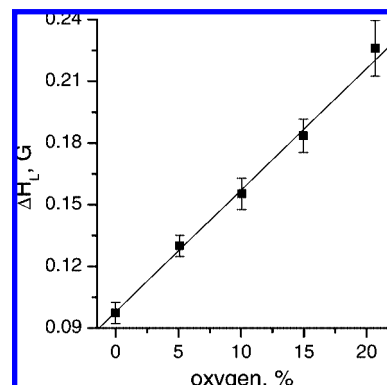
Figure 7. The dependence of Lorentz peak-to-peak line width, \Delta H_L , on oxygen concentration obtained by fitting the calculated spectra of aTAM 4 to the experimental spectra measured at pH 9.9 and pH 5.8 as shown in Figure 6. Within the limits of experimental accuracy the values of \Delta H_L of individual lines of R (pH 9.9) and \text{RH}^+ (pH 5.8) forms were not distinguished. Slope is (6.0 \pm 0.5) mG per % oxygen.
