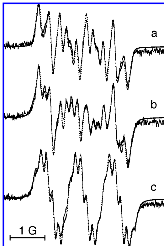
Figure 3. EPR spectra of 10 \mu\text{M} aTAM 5 radical in 1.5 mM N-apyrophosphate buffer under nitrogen atmosphere, 37 °C at pH values 9.40 (a), 8.20 (b), and 6.00 (c). Spectral parameters: microwave power, 0.63 mW; time constant, 163.84 ms; conversion time, 240.0 ms; sweep time, 245.76 s; modulation amplitude, 0.1 G; sweep width, 5 G; number of points, 1024. Dotted lines represent the calculated spectra with peak-to peak line widths, \Delta H_L = 96 mG, \Delta H_G = 95 mG, and following hfs constants: (a) a_N = 0.78 G, a_{D_1}(\text{CD}_2) = 0.15 G, a_{D_2}(\text{CD}_2) = 0.30 G; (c) a_N = 0.99 G, a_{D_1}(\text{CD}_2) = 0.15 G, a_{D_2}(\text{CD}_2) = 0.17 G, a_H(\text{NH}^+\text{Et}_2) = 0.15 G. Calculated spectrum b is a superposition of calculated spectra a (68%) and c (32%) yielding corresponding \text{p}K_a = 7.9 for the protonation of the amino group.
