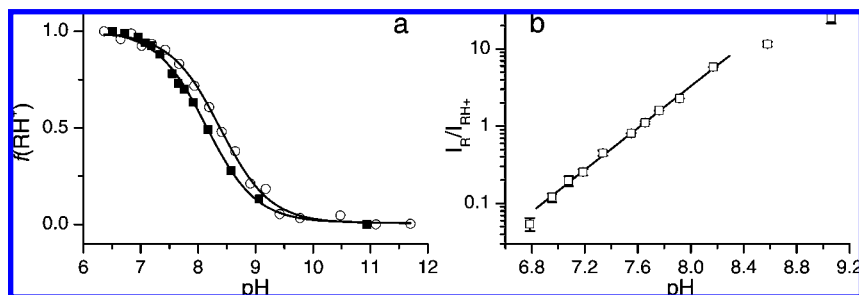
Figure 5. (a) The pH dependence of fraction of aTAM 4 radical protonated form, f_{RH^+} , obtained from EPR spectra measured at 23 °C (○) and 37 °C (□) as shown in Figures 2 and 4. Lines represent the best fits of titration equation to the experimental data yielding pK_a values 8.4 \pm 0.05 (23 °C) and 8.0 \pm 0.1 (37 °C). (b) The pH dependence of spectral amplitude ratios of the high-field components of deprotonated (R) and protonated ( RH^+ ) forms of aTAM 4 radical (see Figure 4a) in logarithmic scale. Lines represent the linear regression, \log(I_R/I_{RH^+}) = a\text{pH} - b , yielding a = 1.35 \pm 0.02 and b = 10.3 \pm 0.2 .
