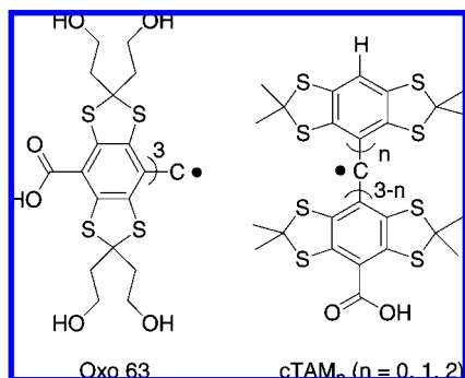
Scheme 1. Chemical structures of Carboxyl Group-Containing TAM Derivatives, Oxo63 and cTAMs a18
