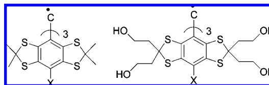
Scheme 3. The Two Basic Structures of TAM-X Radicals with an Ionizable Group, X a
