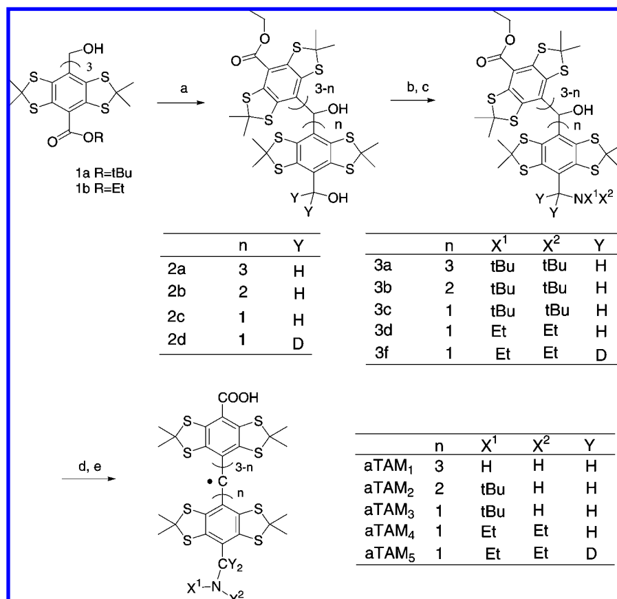
Scheme 2. Synthesis of Dual pH and Oxygen Spin Probes a
