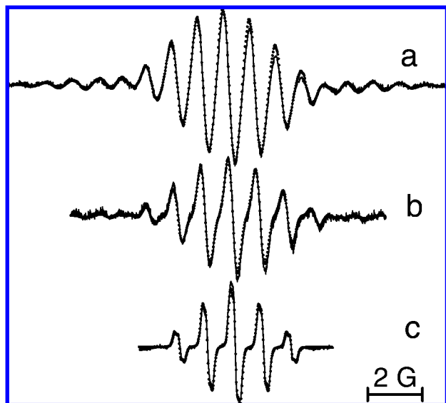
Figure 1. EPR spectra of aqueous solutions of (a) 300 \mu\text{M} aTAM 1 , (b) 150 \mu\text{M} aTAM 2 , and (c) 30 \mu\text{M} aTAM 3 , pH 5.0, under nitrogen atmosphere and at 37 °C. Spectral parameters were as follows: microwave power, 0.63 mW; time constant, 20.48 ms; conversion time, 160 ms (a, b) and 80.00 ms (c); sweep time, 327.68 s (a, b) and 81.92 s (c); modulation amplitude, 0.1 G; sweep width 20 G (a, b) and 8 G (c); number of points, 2048 (a, b) and 1024 (c). Dotted lines represent the simulated spectra with the values of peak-to-peak line widths, \Delta H_L = 97 mG and \Delta H_G = 94 mG, and following hfs constants: (a) a_N = 0.96 G, a_{H_1}(\text{CH}_2) = 0.97 G, a_{H_2}(\text{CH}_2) = 1.02 G, a_{H_3-H_5}(\text{NH}_3^+) = 0.13 G, and a(^{13}\text{C}) = 6.79 G; (b) a_N = 0.98 G, a_{H_1}(\text{CH}_2) = 0.99 G, a_{H_2}(\text{CH}_2) = 1.04 G, a_{H_3-H_4}(\text{NH}_2^+t\text{-Bu}) = 0.13 G, and a(^{13}\text{C}) = 7.2 G; (c) a_N = 1.02 G, a_{H_1}(\text{CH}_2) = 0.97 G, a_{H_2}(\text{CH}_2) = 1.04 G and a_{H_3-H_4}(\text{NH}_2^+t\text{-Bu}) = 0.13 G.
