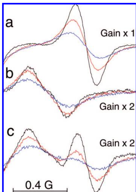
Figure 6. High-field components of the EPR spectra of aTAM 4 measured in 1.5 mM pyrophosphate buffer, pH 9.9 (a), pH 5.8 (b), and pH 7.8 (c), at various oxygen partial pressures: 0% (black), pH 5.8 (red), 20.7% (blue). Spectral parameters: microwave power, 0.63 mW; time constant, 40.96 ms; conversion time, 160 ms; sweep time, 327.68 s; modulation amplitude, 0.1 G; sweep width, 8 G; number of points, 2048. Experimentally measured peak-to-peak line widths are \Delta H_{pp} = 160 mG (a) and \Delta H_{pp} = 280 mG (b). Fitting the calculated spectra to the experimental spectra a and b at 0% oxygen using hfs given in the caption to Figure 2 and describing individual line shape by convolution of Lorentz and Gauss profiles 22 yields the following peak-to-peak line widths: (a) \Delta H_L = 96 mG, \Delta H_G = 100 mG, and (b) \Delta H_L = 97 mG, \Delta H_G = 94 mG. Note that the values of the obtained parameters for the nonprotonated radical (a) are in agreement with the previously reported equation for convolution of Lorentz and Gauss profiles ( \Delta H_L/\Delta H_{pp} + \Delta H_G^2/\Delta H_{pp}^2 = 1 ). 22 This is not valid for the protonated form of the radical (b) due to the fact that \Delta H_{pp} represents peak-to-peak line width of partially unresolved doublet aroused from additional proton hfs, a_H(\text{NH}^+\text{Et}_2) = 0.15 G (Figure 2). Fitting the calculated spectra of R and \text{RH}^+ forms to the experimental spectra a and b, respectively, measured at various concentration of oxygen yield the values of \Delta H_L shown in Figure 7. Fitting the calculated spectra to the experimental spectra c measured at intermediate pH and various concentrations of oxygen yields the values of peak-to-peak line width, \Delta H_L , and fraction of protonated form, f_{\text{RH}^+} , allowing simultaneous [\text{O}_2] and pH determination using corresponding calibration curves (Figures 7 and 5a, respectively), namely: (black) \Delta H_L = 105 mG (1.3%), f_{\text{RH}^+} = 0.58 (pH 7.85); (red) \Delta H_L = 166 mG (11.3%), f_{\text{RH}^+} = 0.57 (pH 7.88); (blue) \Delta H_L = 227 mG (21.5%), f_{\text{RH}^+} = 0.62 (pH 7.8). The latter examples demonstrate an accuracy in pH ( \pm 0.1 ) and oxygen ( \pm 2\% ) determination using aTAM 4 probe in the range of pH around its pK_a .
