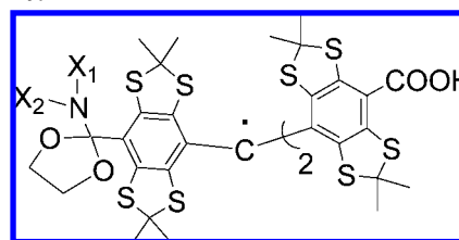
Scheme 4. Hypothetical Structure of aTAM with an Acetal Moiety a
